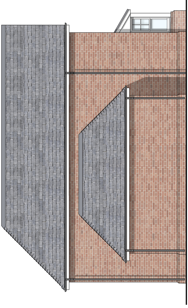
SOUTH EAST ELEVATION
